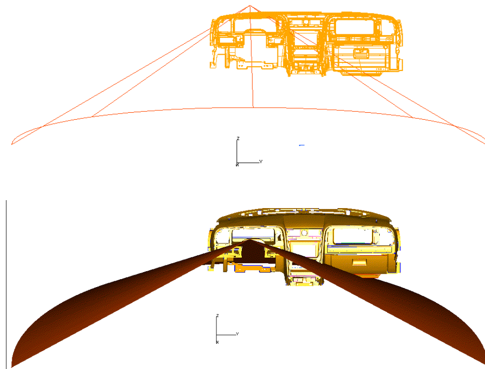
Fig 10. Rear view of same cone and instrument panel as in Fig. 9. The top picture is a wire frame view, and the bottom picture is a solid view, with the rear portion of the cone cut away so the interior can be seen.
